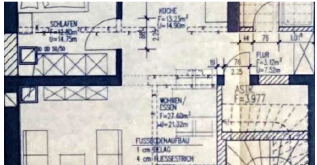
Grundriss WHG 1.OG links
