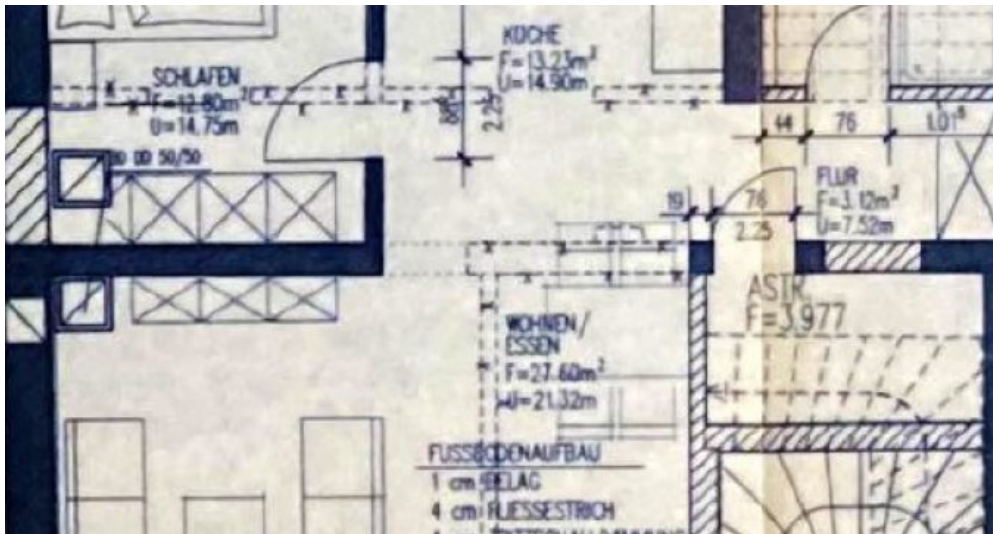
Grundriss WHG 1.OG links
