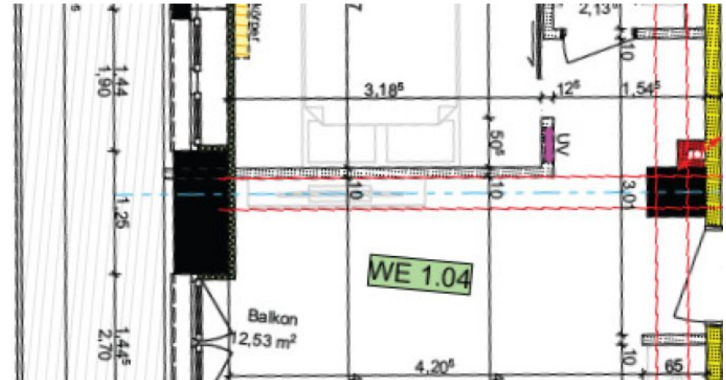
Grundriss WHG 1.04
